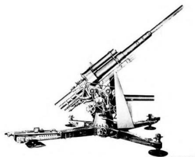
Figure 1 — German 88-mm Antiaircraft Gun — Firing Position
